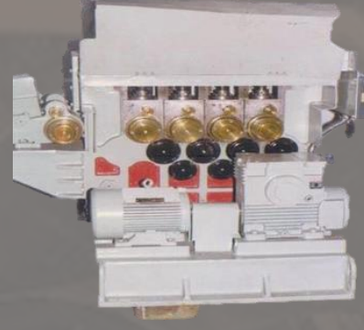
Straightening M/c
