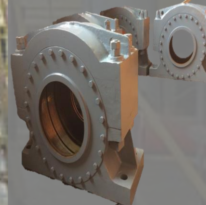
Bearing Housing
